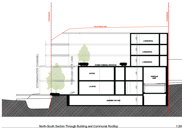
North-South Section Through Building and Communal Rooftop
