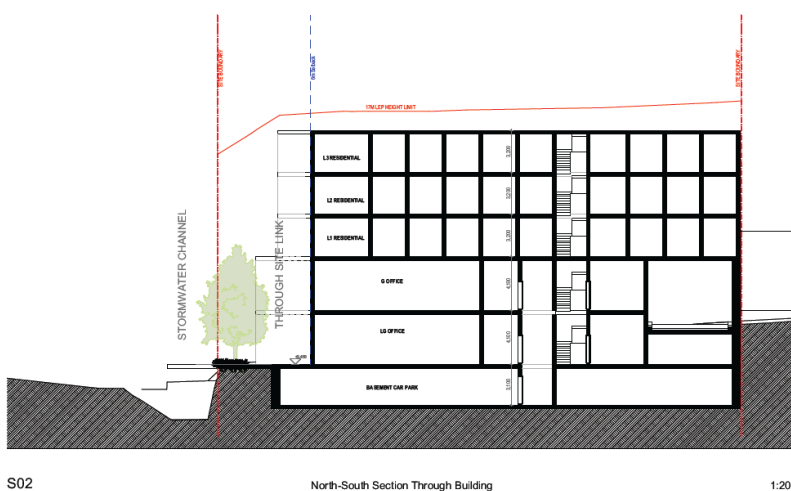
Figure 8 - North-South Section through the building indicating 6m setback from the creek and 17m (5 storey) height limit
