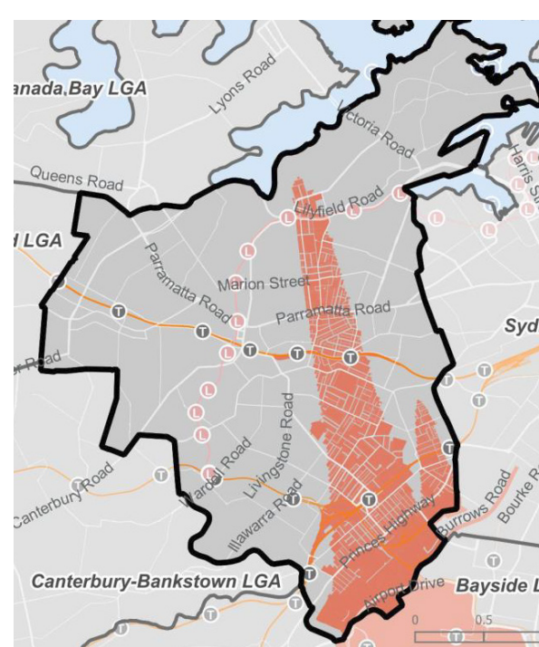
Aircraft noise
