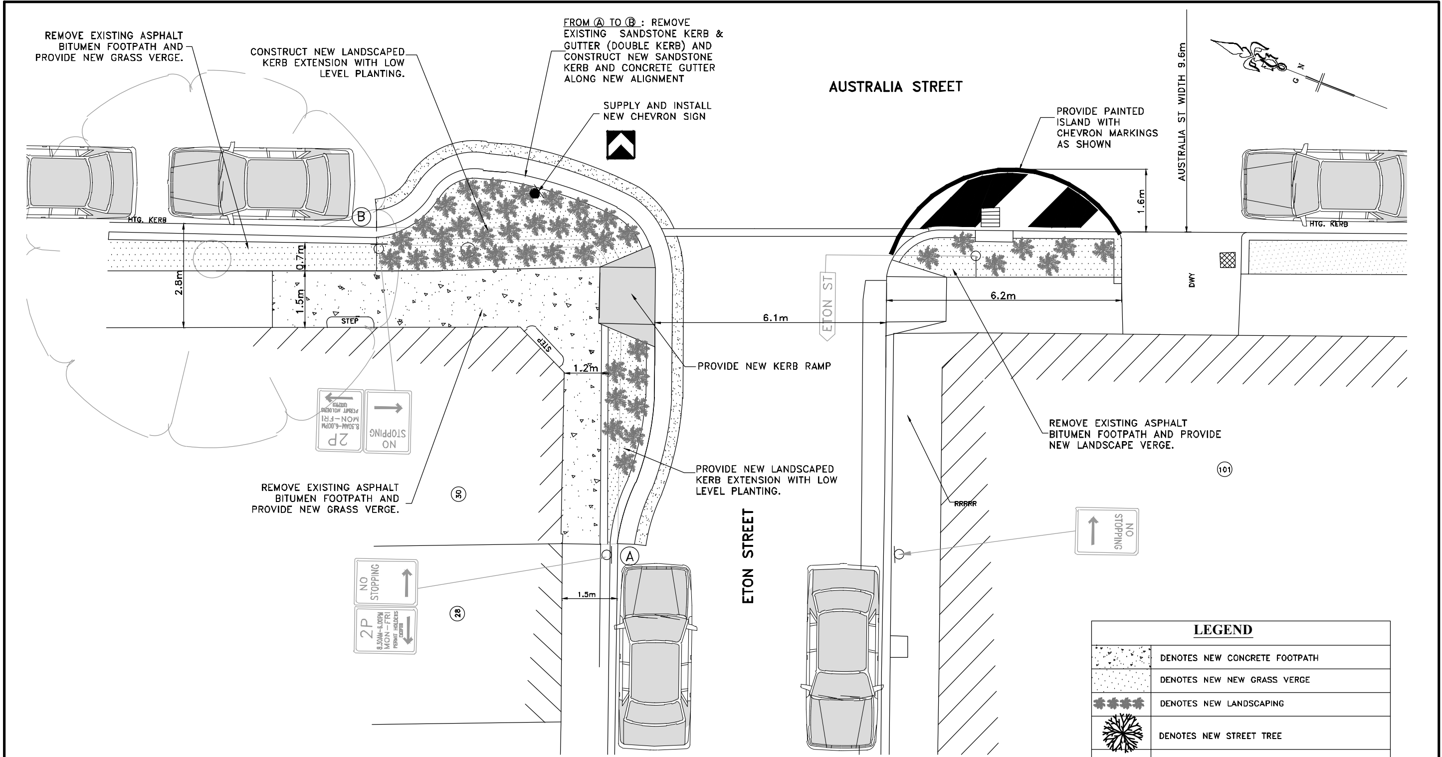
GENERAL LAYOUT SCALE 1:50
